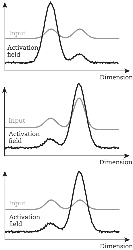
FIGURE 2.10: Input functions (solid gray lines) and stable activation patterns (solid black lines) are shown as functions of the field dimension in three situations. Top: Input is bimodal, with identical maximal level of input at two locations. An activation peak centered on the left mode is a stable state that may have emerged because activation was initially higher on the left from the leftmost mode being presented first, or by chance from fluctuations in input. Middle: When input to the rightmost location is much stronger than to the leftmost location, the peak centered on the left location is no longer stable and the system switches in selection instability to a peak centered on the rightmost location. Bottom: If input is then returned to symmetric levels for both modes, the peak centered on the right mode remains stable, an instance of the stabilization of selection decisions.
