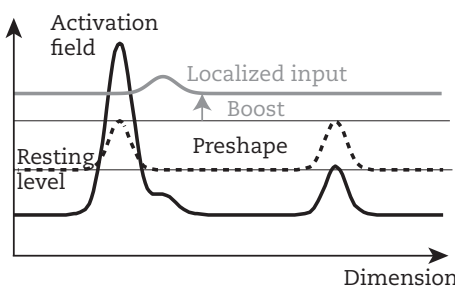
FIGURE 2.13: Categorical responding based on the memory trace: A field is preshaped (dashed line) by a memory trace at two locations at which peaks of activation have been frequently encountered. Other regions of the field are at resting level. When a weak localized input is applied jointly with a boost to the field (gray solid line), a self-stabilized peak (black solid line) is generated at the preactivated location that best overlaps with the small, localized input. Elsewhere, the field is suppressed below resting level, including at the precise location of the small, localized input.
